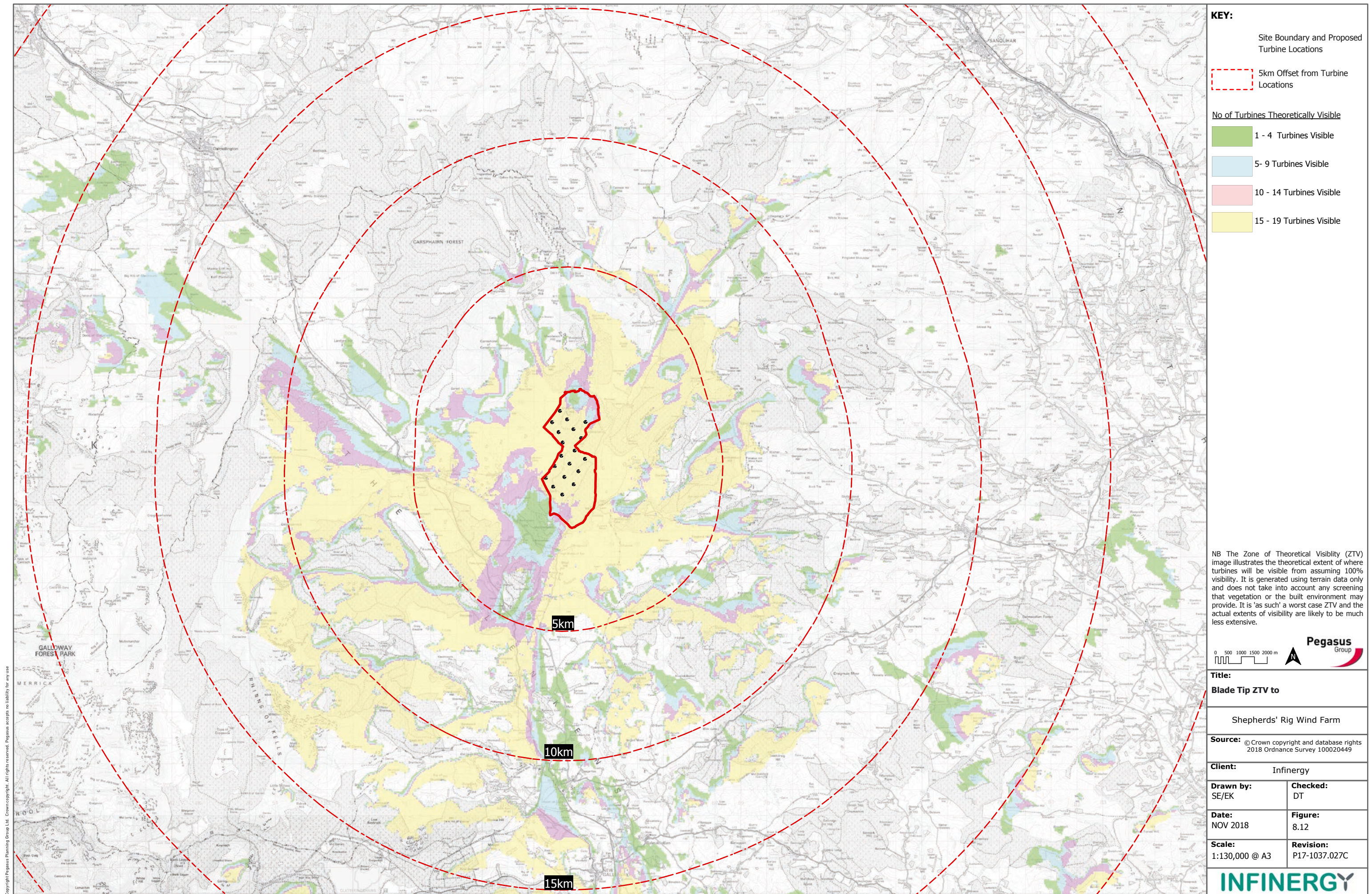
Figure 8.12: Blade Tip ZTV to 15 km
